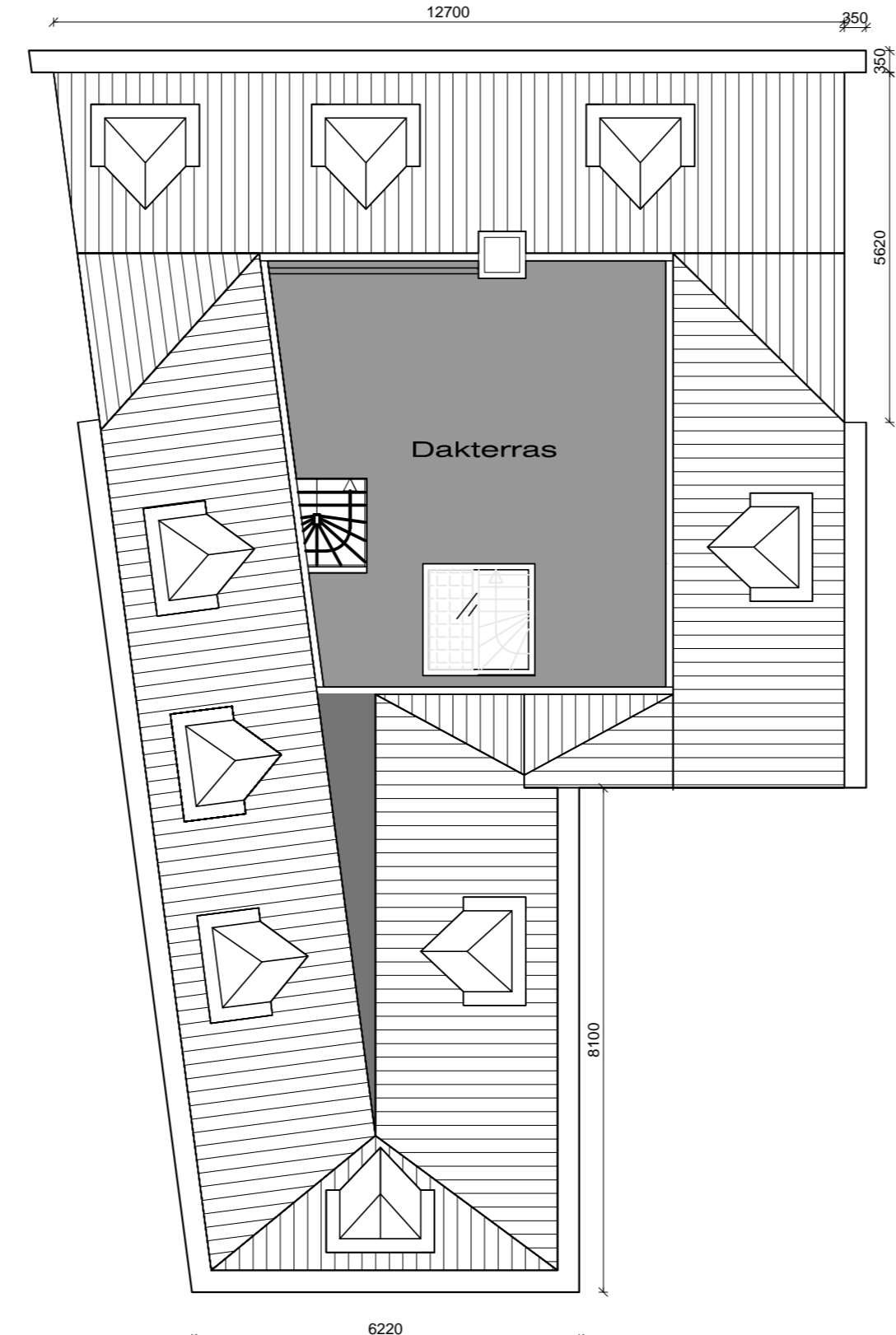
Dakplan
